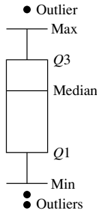
Figure 12.3 Using a boxplot to visualize outliers.
