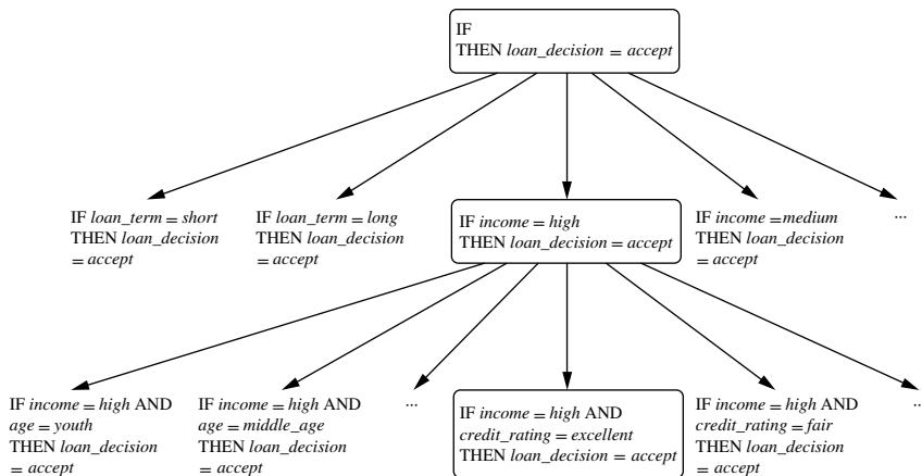
Figure 8.11 A general-to-specific search through rule space.
